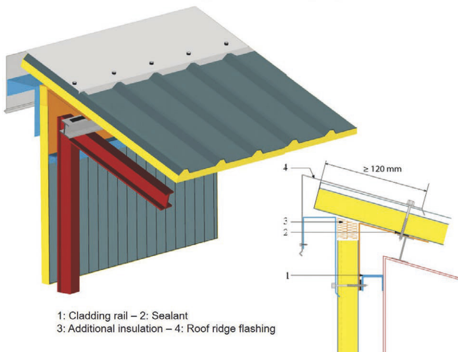
Detail 36: Monorooft ridge with overhang beyond wall
