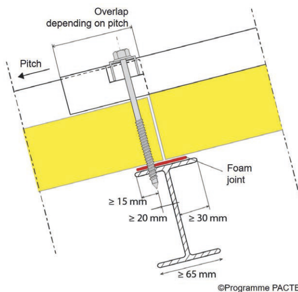
Figure 26: Special conditions flush with the overlapping panel ends (see table 10)
