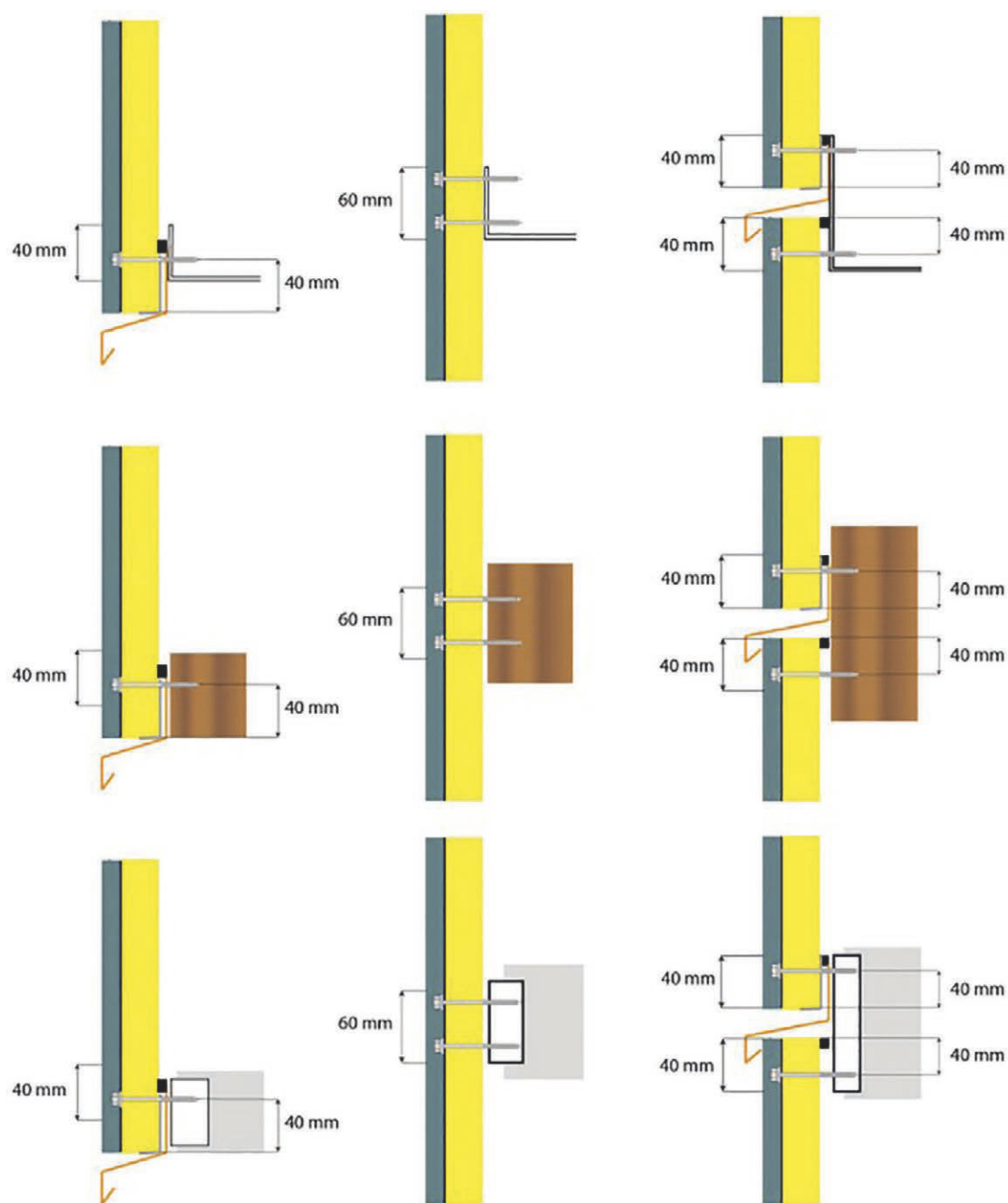
Figure 23: Examples of edge distances for wall panels with hidden fixings installed vertically on different types of support
