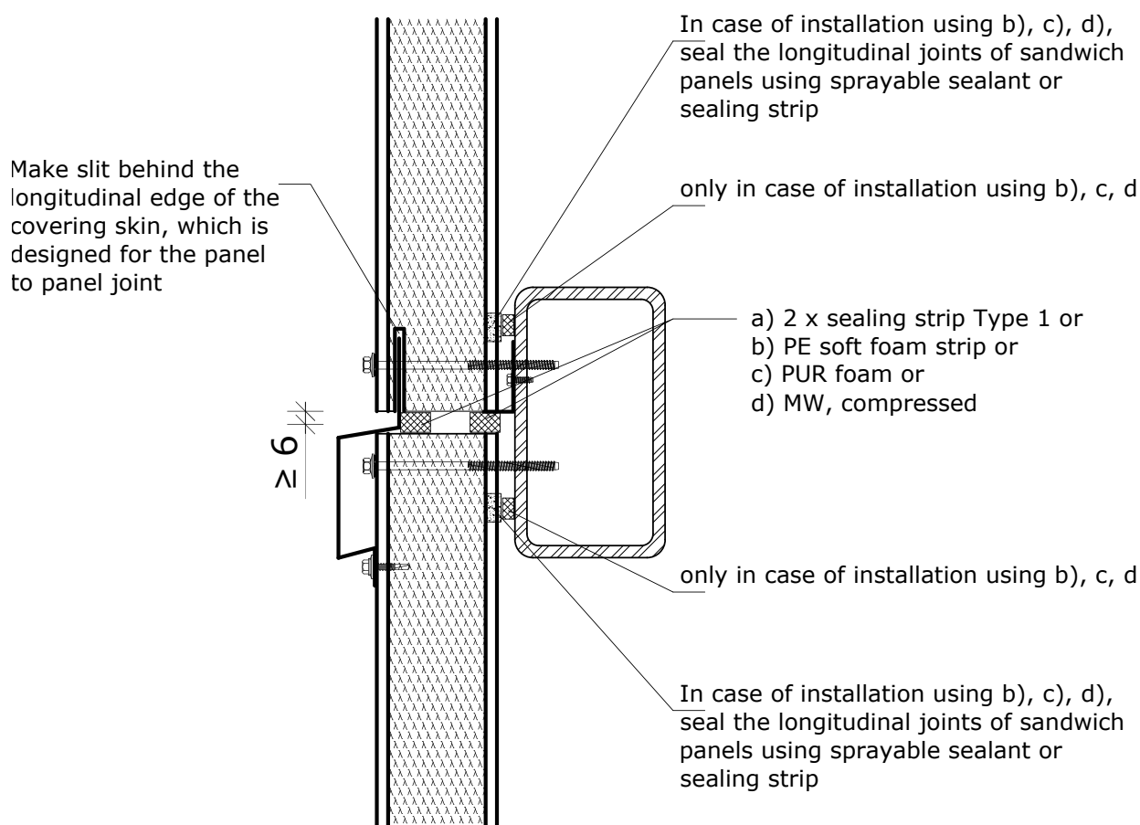
Figure 49: Detail of end-to-end wall panel joints in Germany
