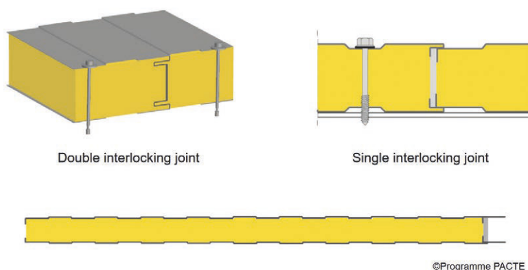
Figure 1a: Example of sandwich panels with visible through-fixings and single or double interlocking joints
