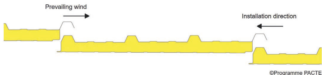
Figure 40: Installation direction
