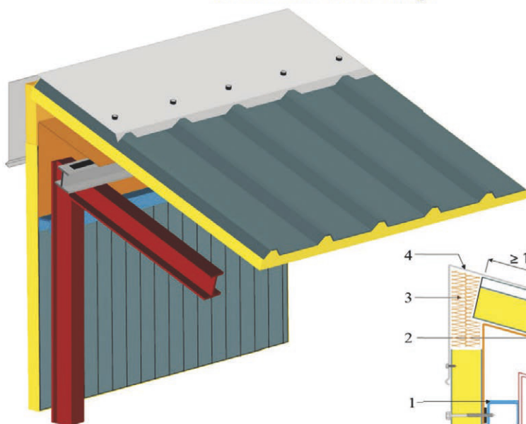
Detail 34: Monorooft ridge
