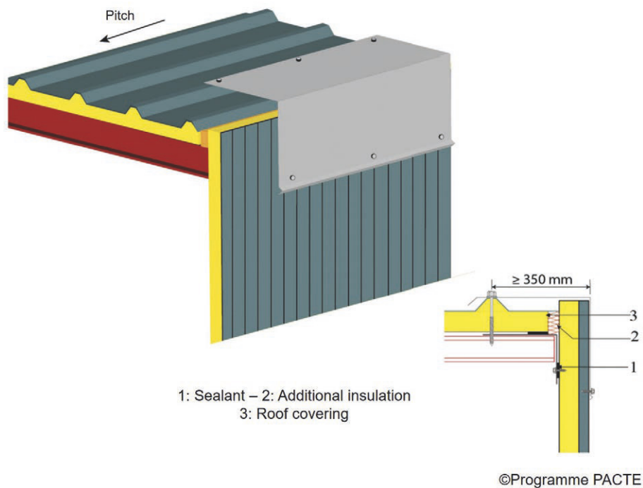
Detail 38: Verge flashing
