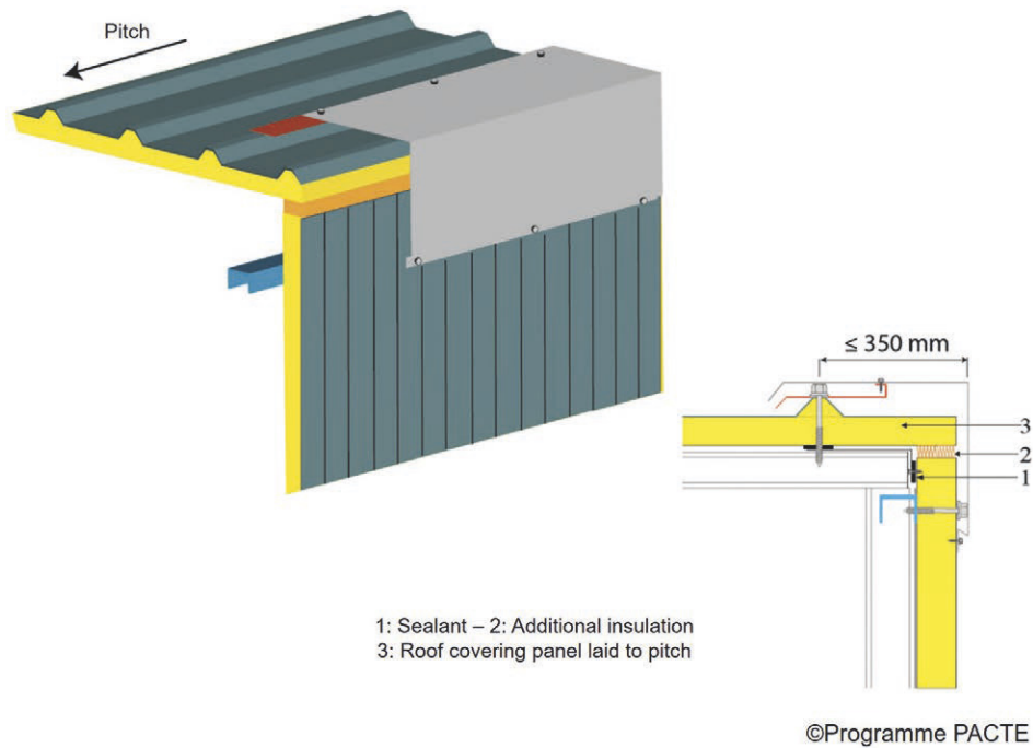
Detail 24: Top of cladding – Vertically installed panels
