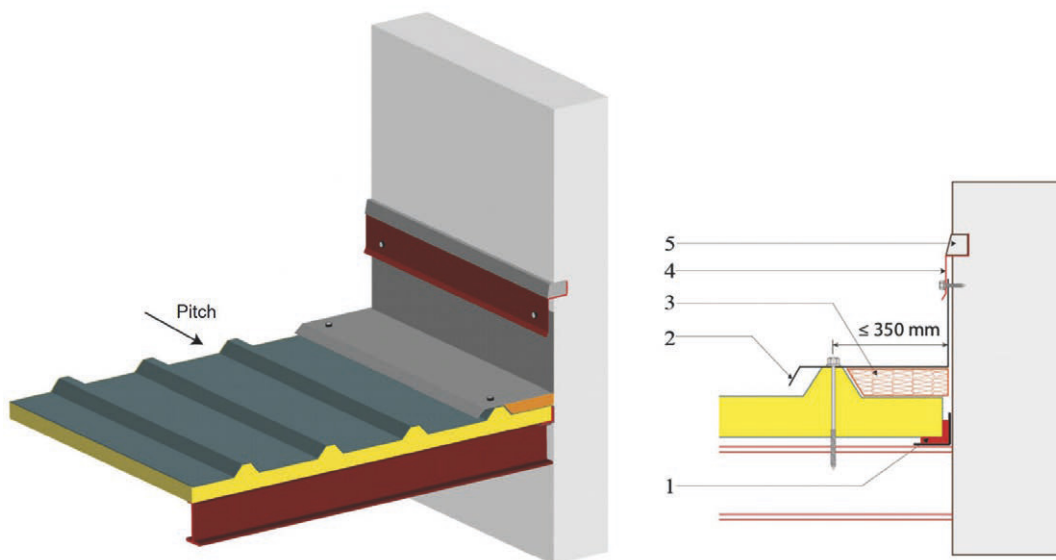
Detail 37: Wall abutment
