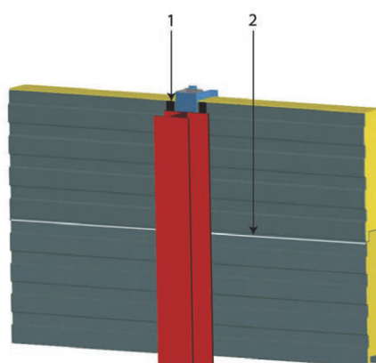
1: Silicone joint on support 2: Silicone gasket at longitudinal joints between panels
