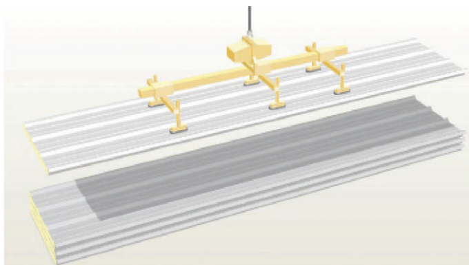
Figure 31: Handling using spreader bar with vacuum cups
