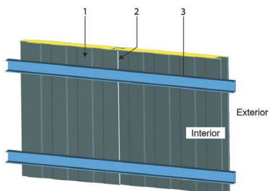
1: Panel 2: Silicone gasket at longitudinal joints between panels 3: Cladding rail
