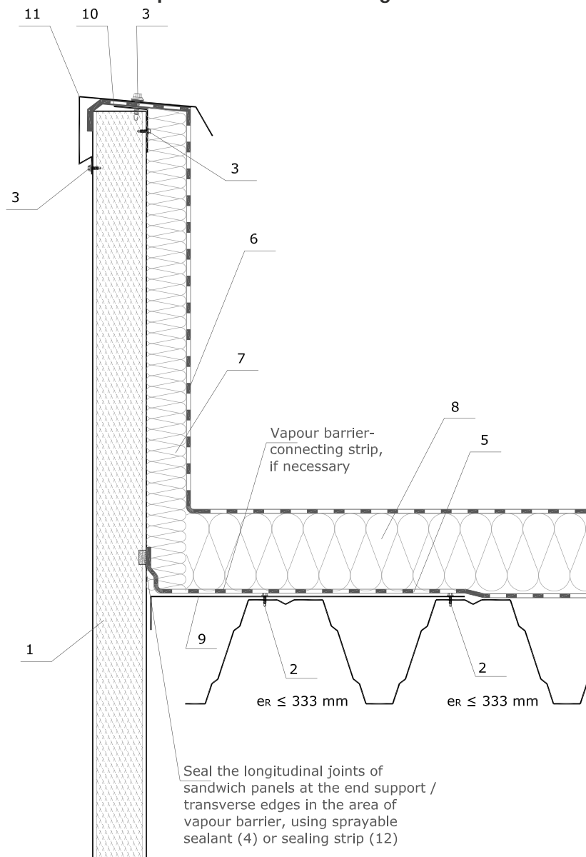
Detail 29: Parapet with vertical cladding – Construction detail recommended in Germany
