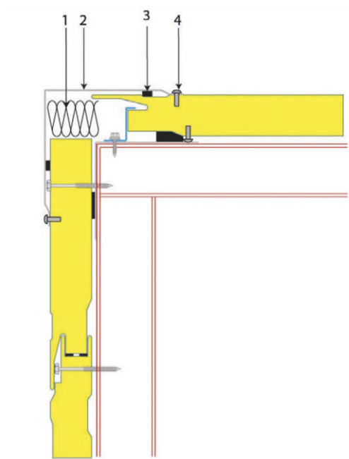
1: Additional insulation – 2: External corner flashing 3: Sealing strip – 4: Rivet or screw
