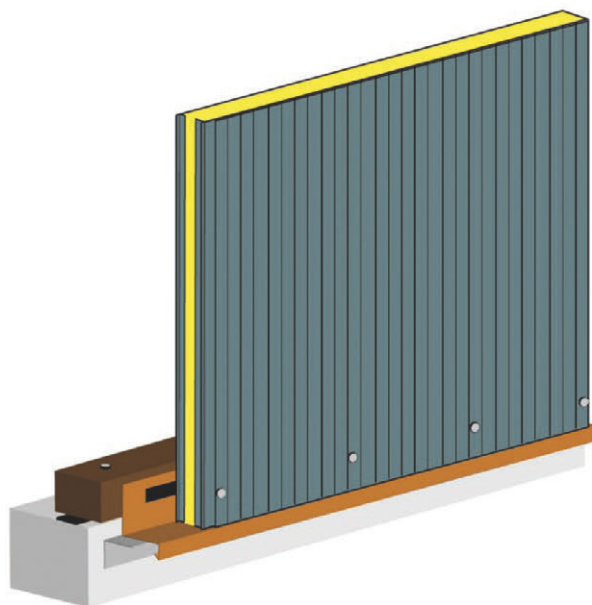
1: Apron (optional) – 2: Anchor 3: Timber support – 4: Sealant
