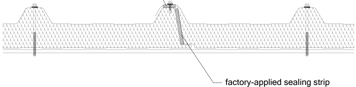
Figure 50: Sealing solution for roof panel side laps in Germany
