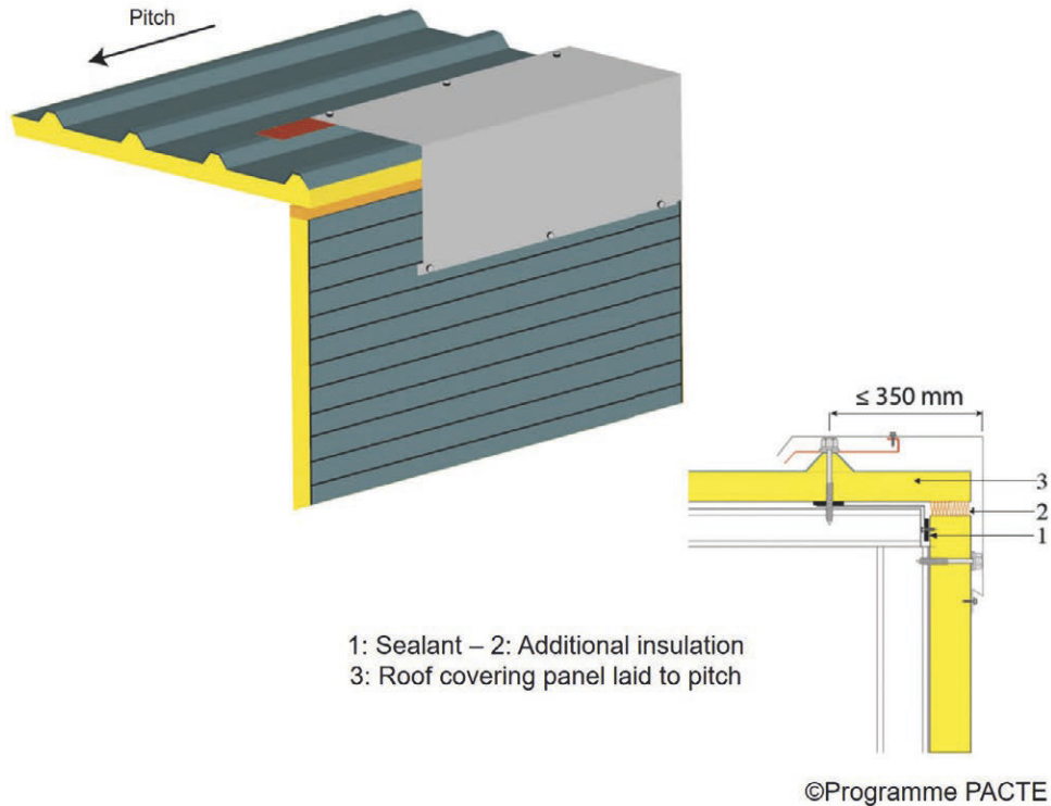
Detail 23: Top of cladding – Horizontally installed panels
