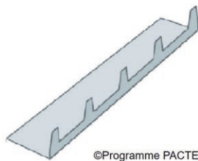
Figure 9: Profile closer flashing
