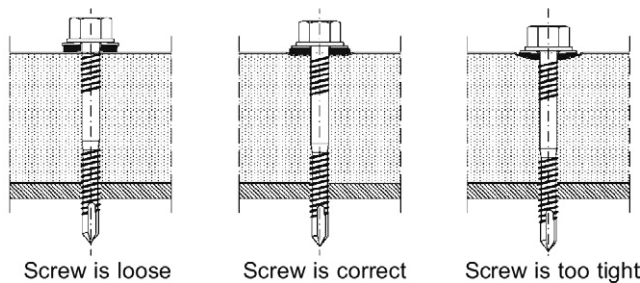
Figure 17: Seating of screws and sealing washers
