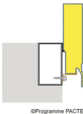
Figure 22: Example of support detail for wall panels with hidden fixings
