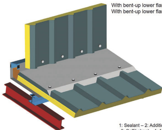
Detail 33: Wall abutment at top of slope – Case 2
