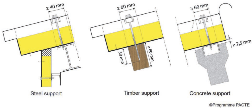
Figure 24: End support conditions
