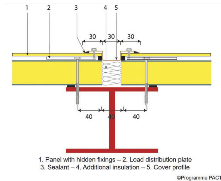
Figure 21: Example of support detail and edge distances for wall panels with hidden fixings installed horizontally on a common steel support
